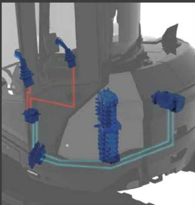
E.O.C. WORLD MOST ADVANCED HYDRAULICS SYSTEM Electronic Open Center (E.O.C.) cuts fuel usage and boosts productivity and controllability, including on AUX lines. Standard from CX60D.
